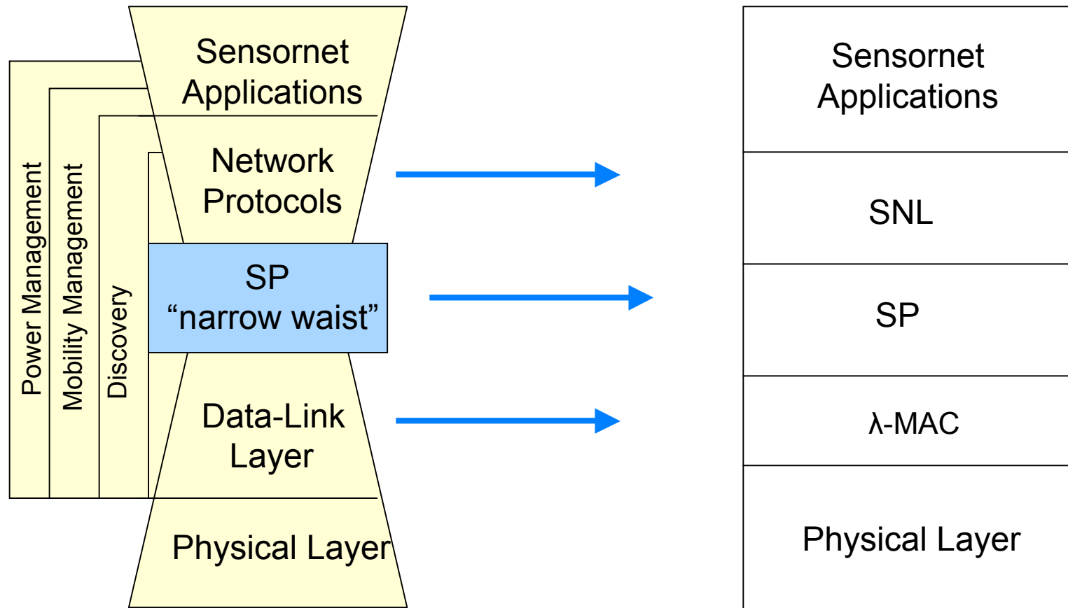
Sensornet Protocol Stack (SP Architecture)
